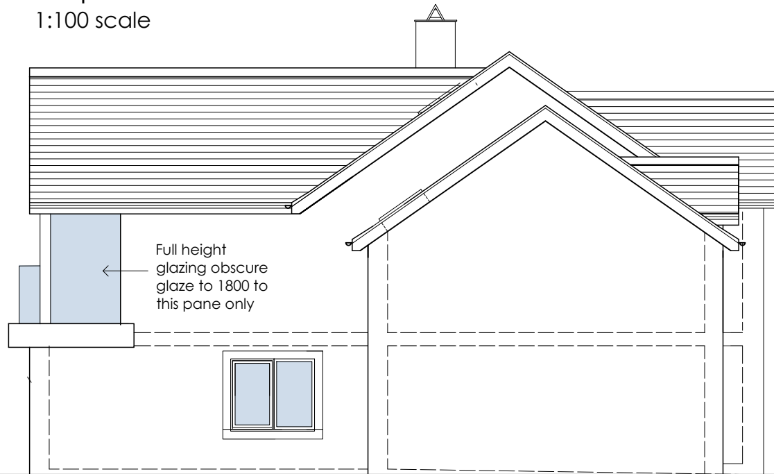
North West Facing Side Elevation
