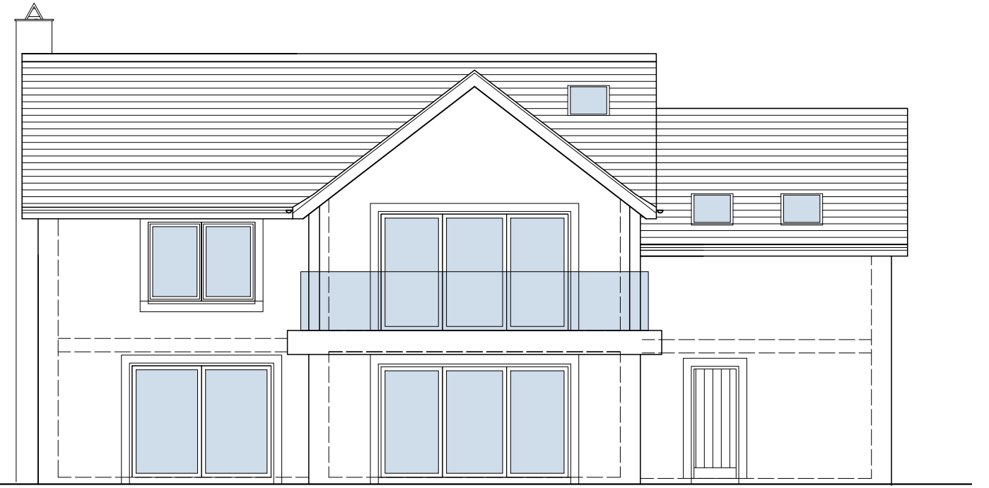
Rear Elevation North East Elevation
