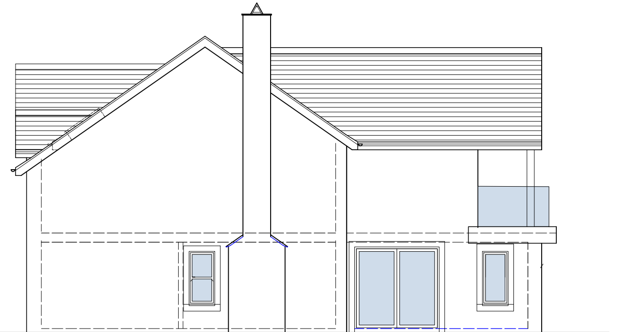
South East Facing Side Elevation
